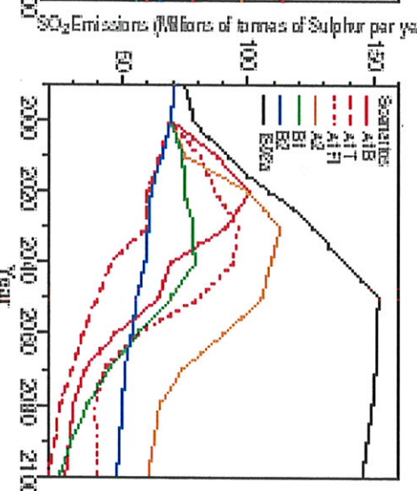
(c) SO 2 emissions
