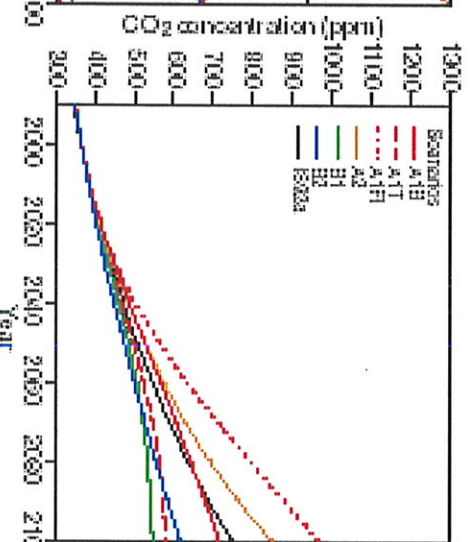
(b) CO 2 concentrations
